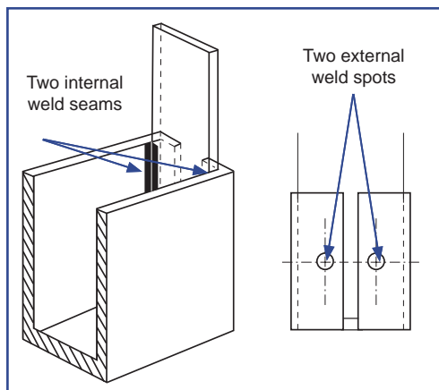
Strap fixing on support
